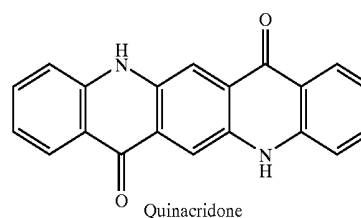
Quinacridone
